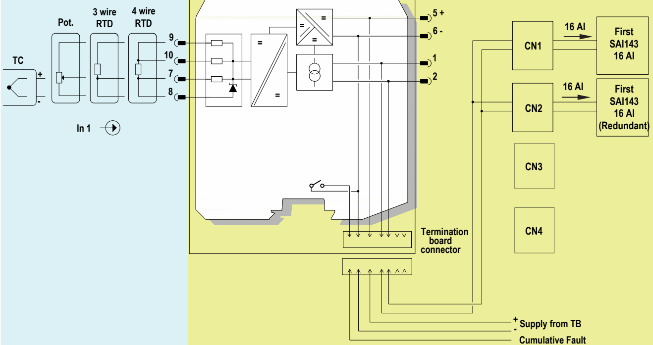
TB position 1 to 16 for single channel Temperature module
