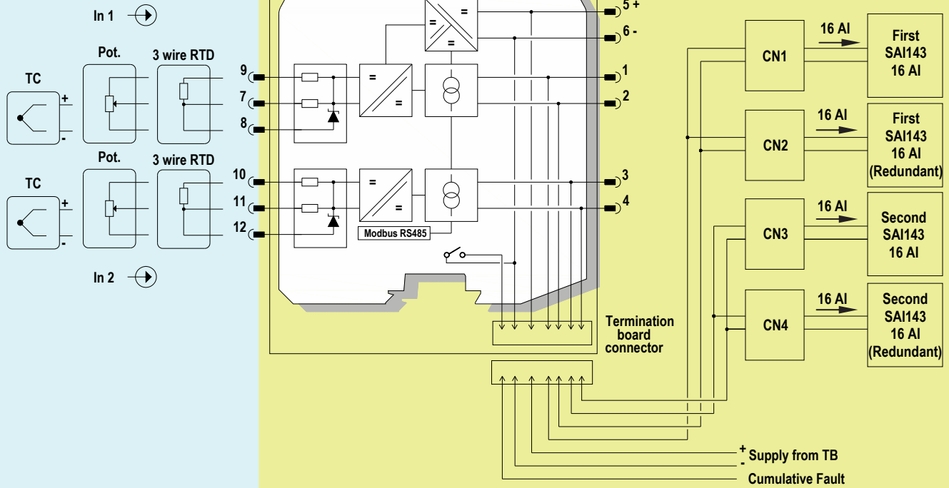
TB position 1 to 16 for double channel Temperature module
