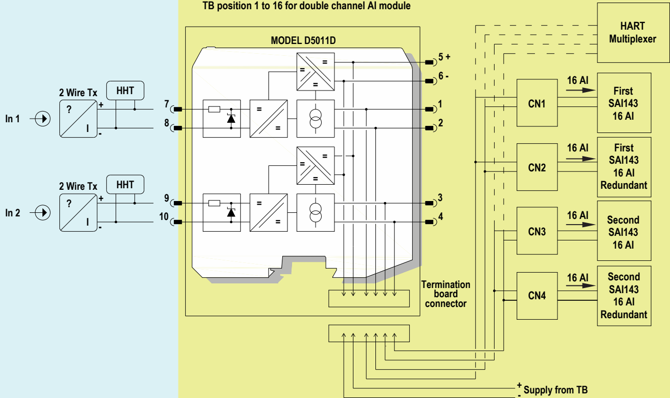
TB position 1 to 16 for double channel AI module
