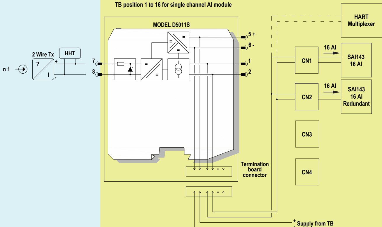
TB position 1 to 16 for single channel AI module
