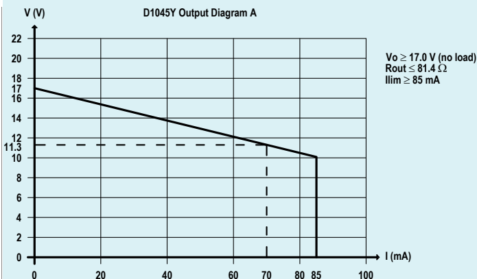
D1045Y OUTPUT DIAGRAM OUT A
